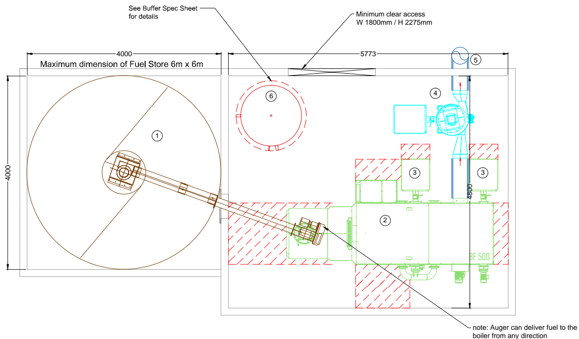
Plan View
