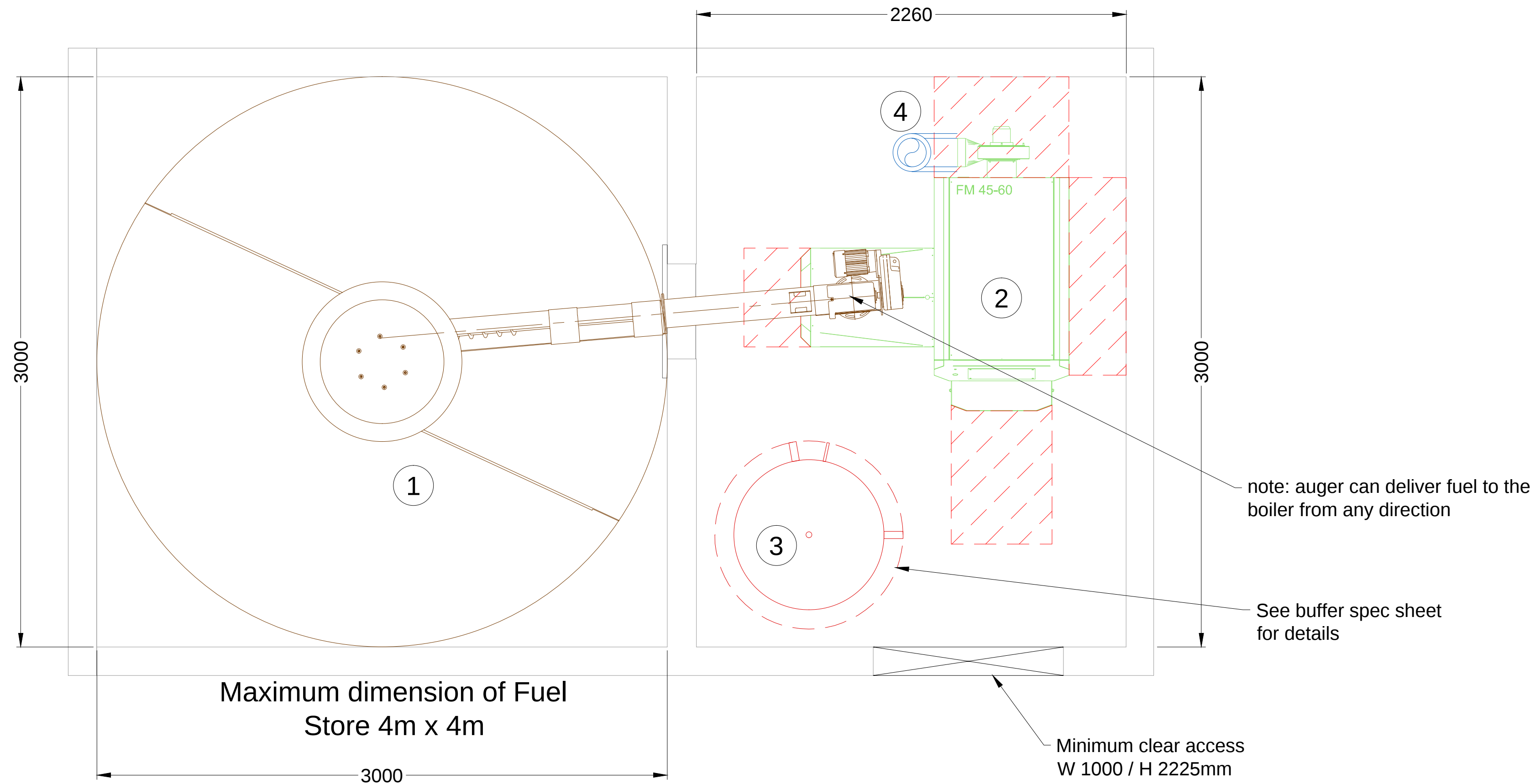
Plan View
