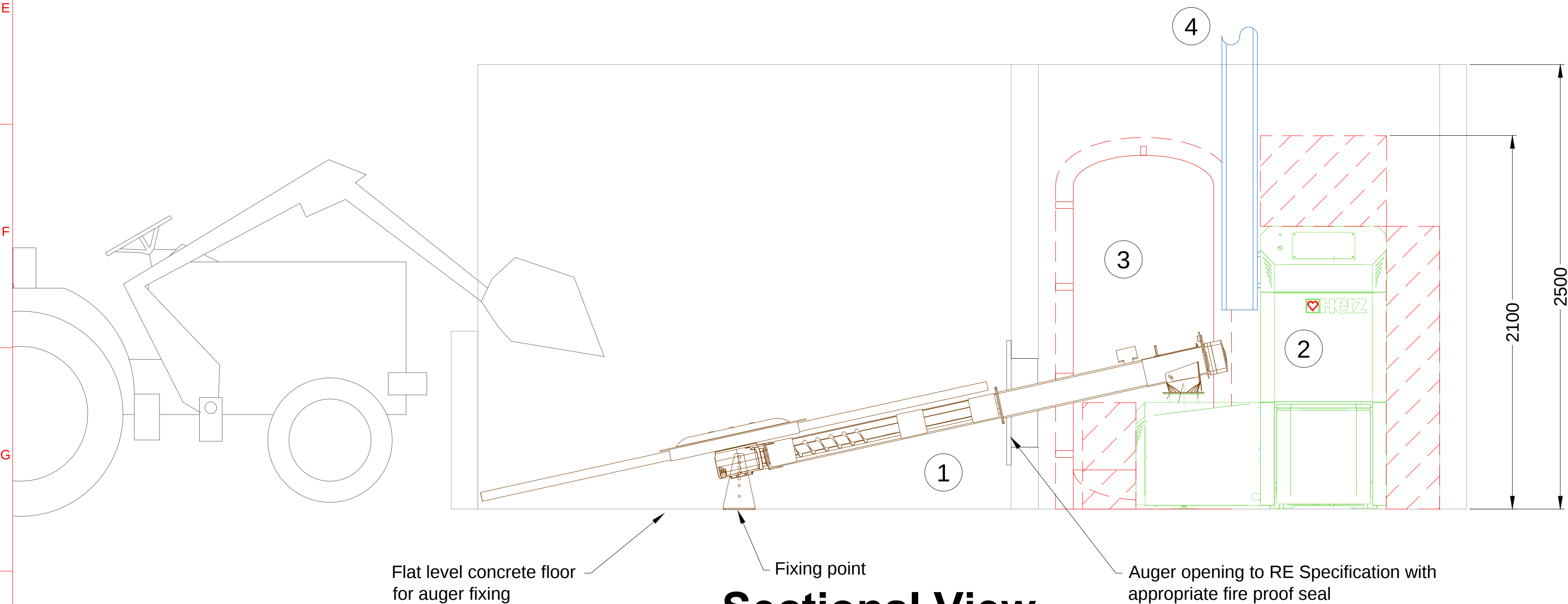
Sectional View
