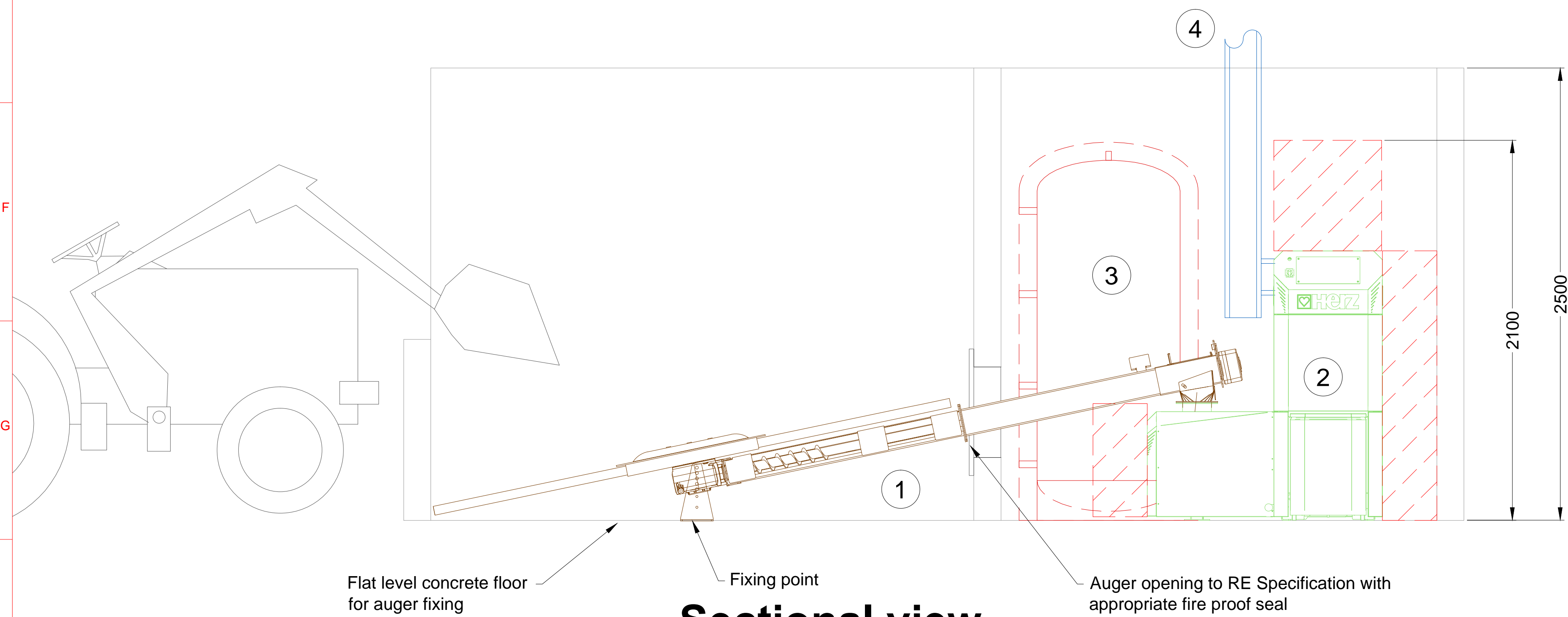
Sectional view
