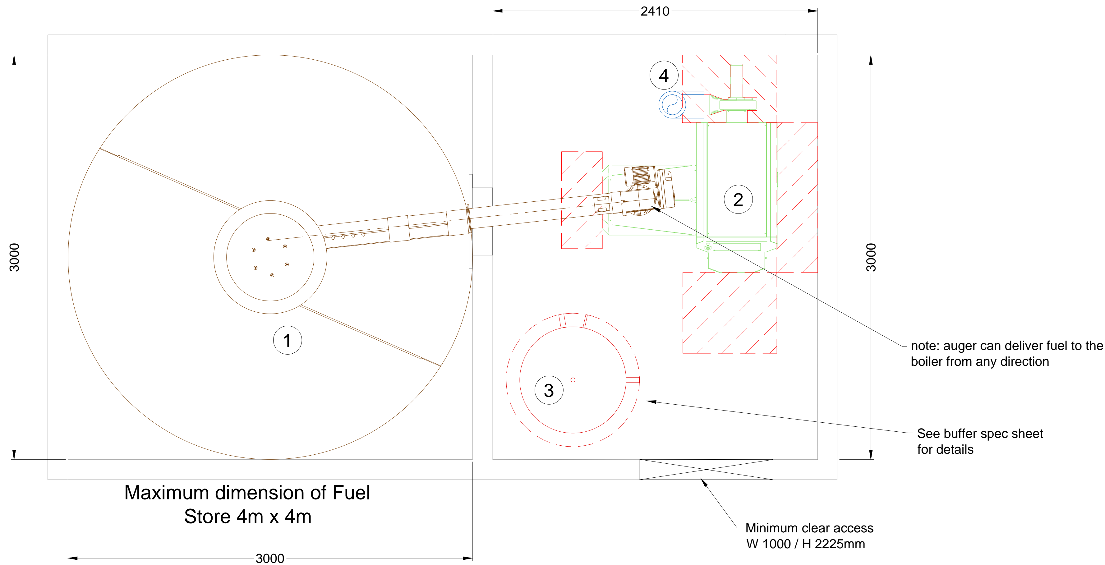
Plan View
