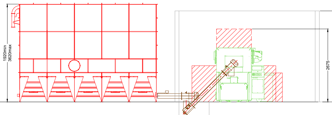
Sectional View
