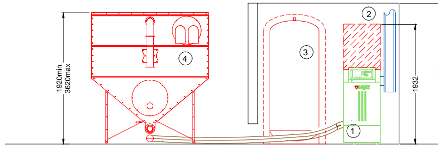
Sectional View
