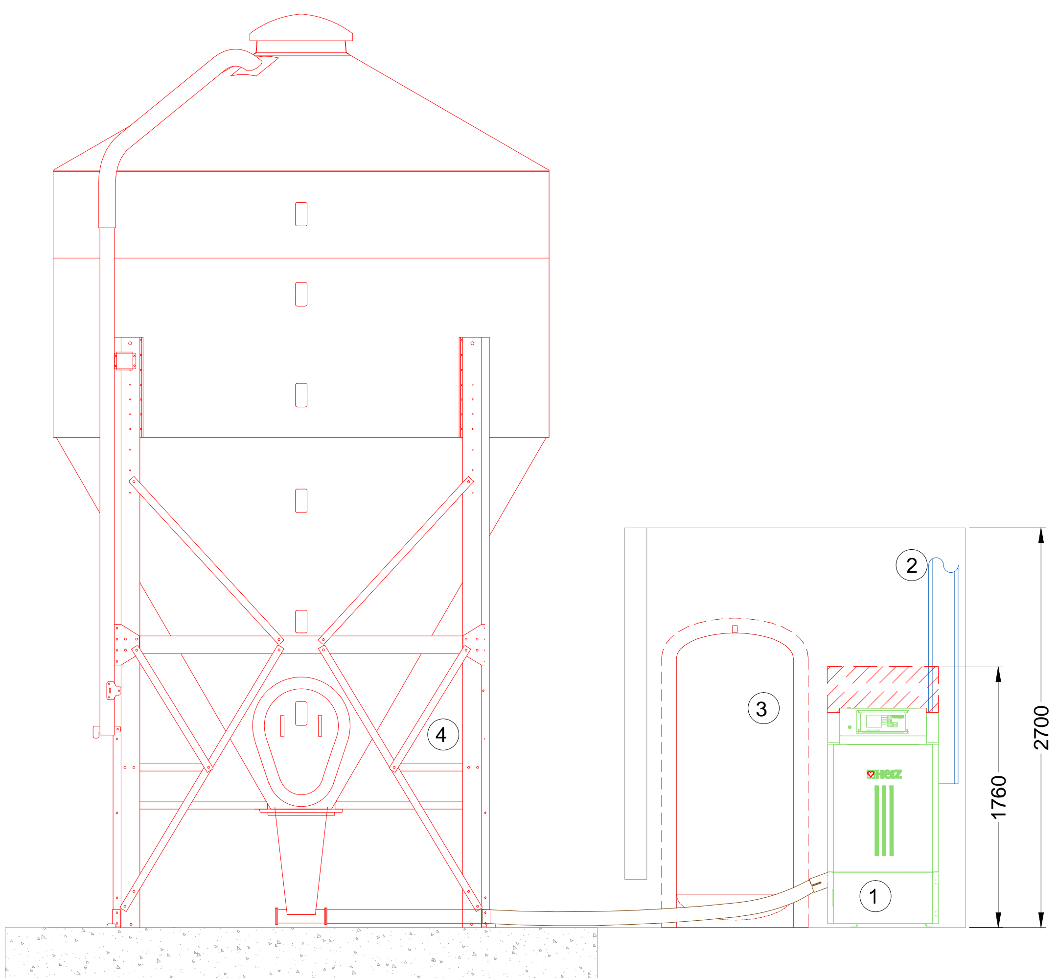
Sectional View
