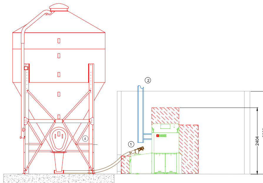
Sectional View
