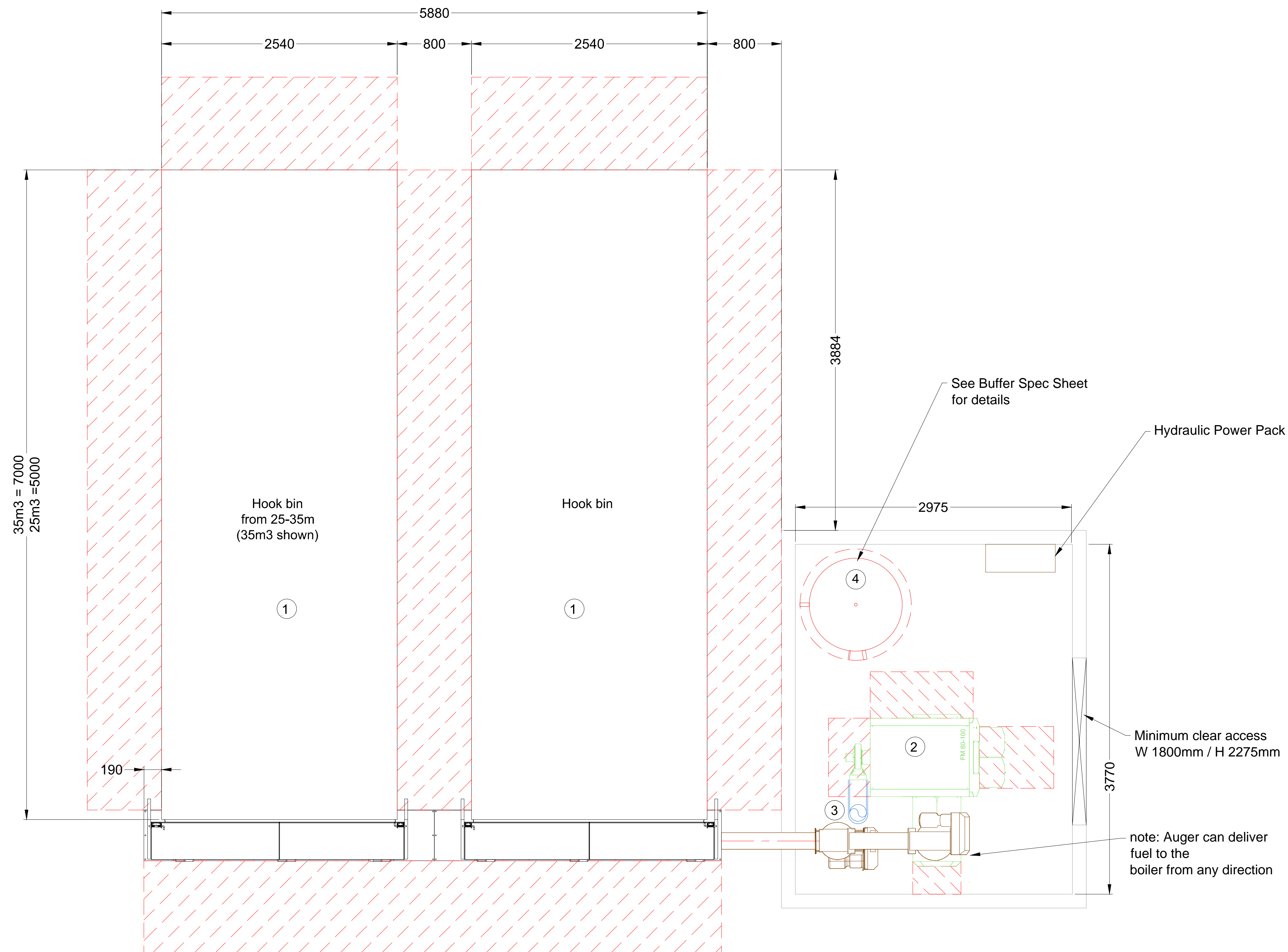
Plan View
