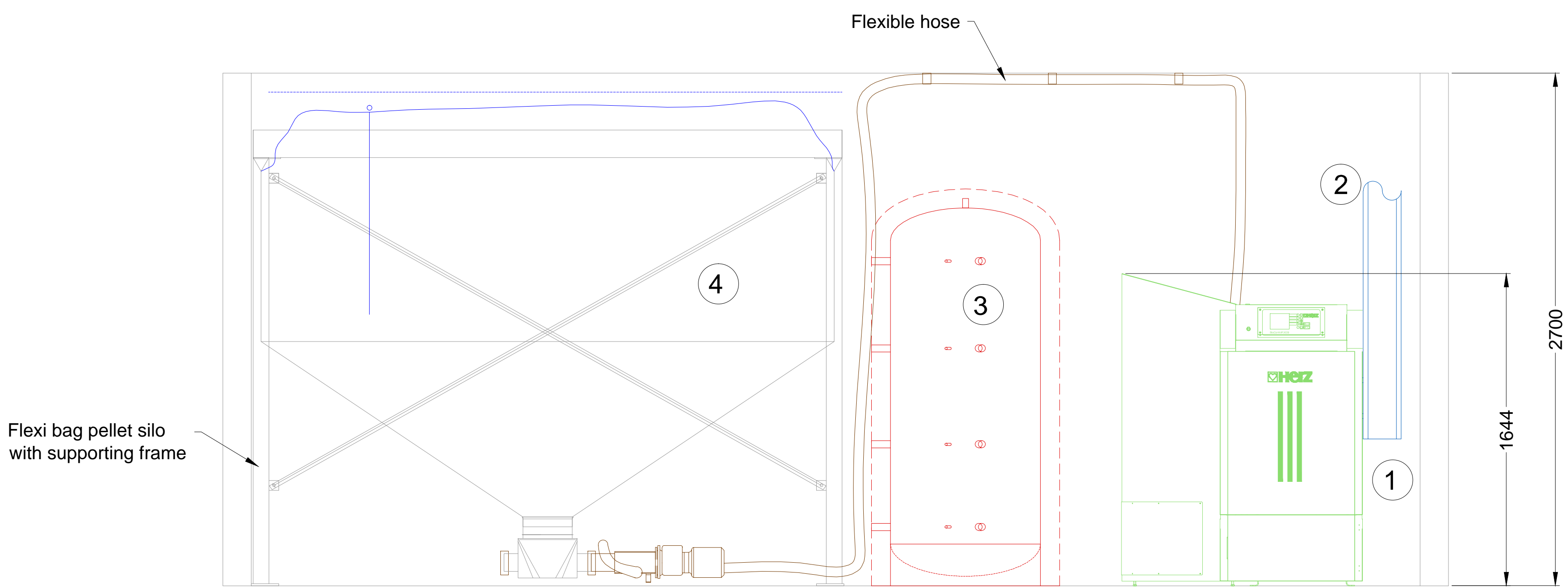
Sectional View
