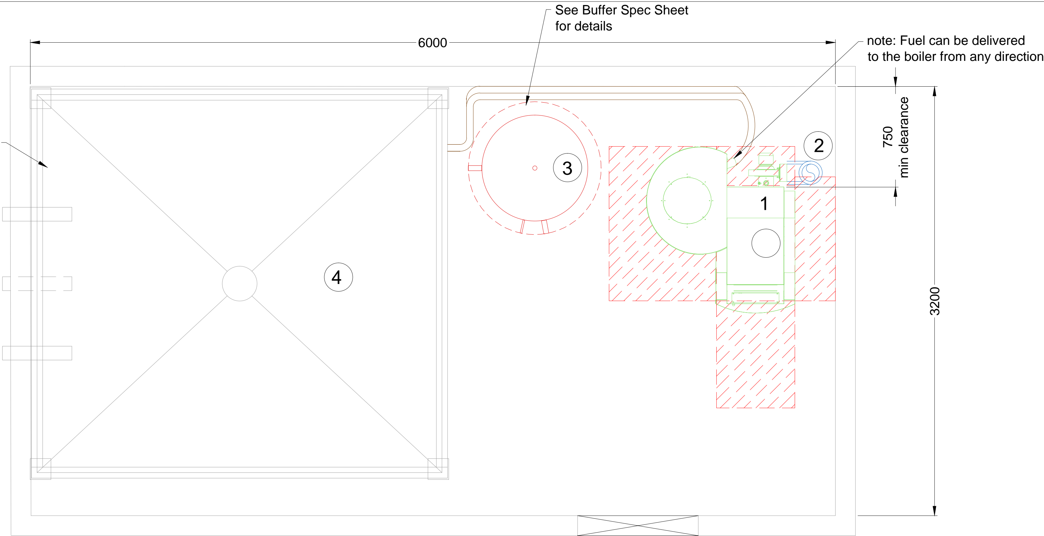
Plan View
