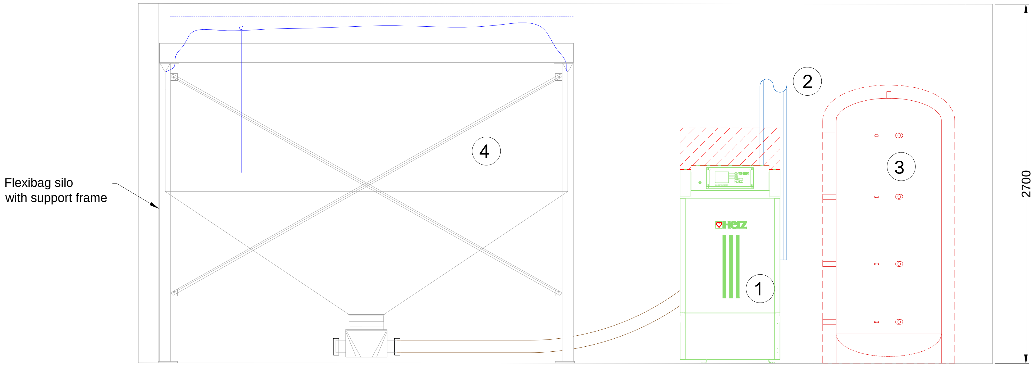
Sectional View
