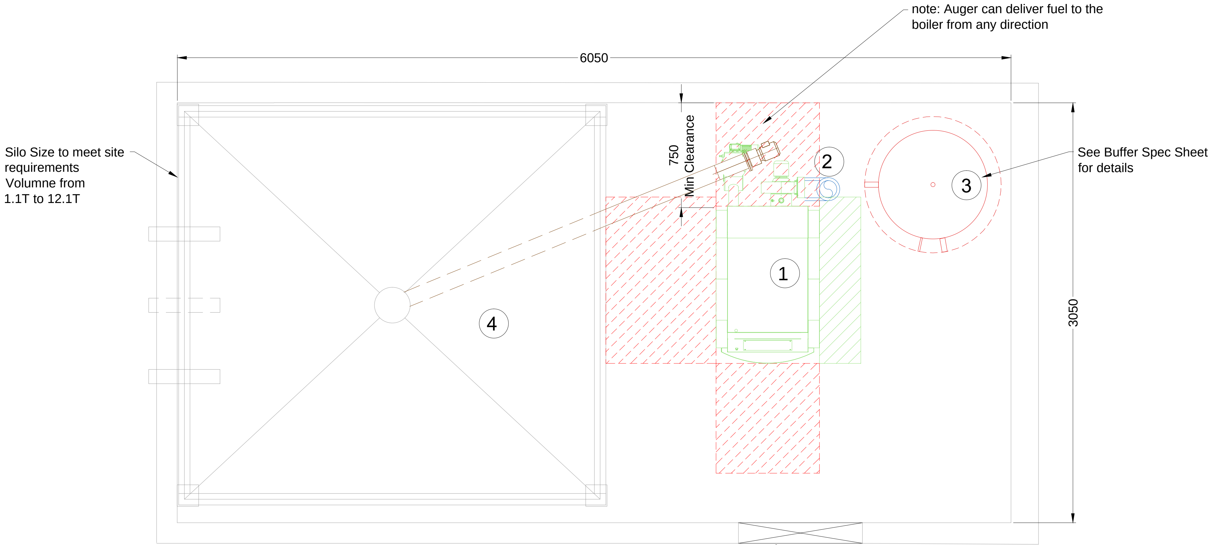
Plan View
