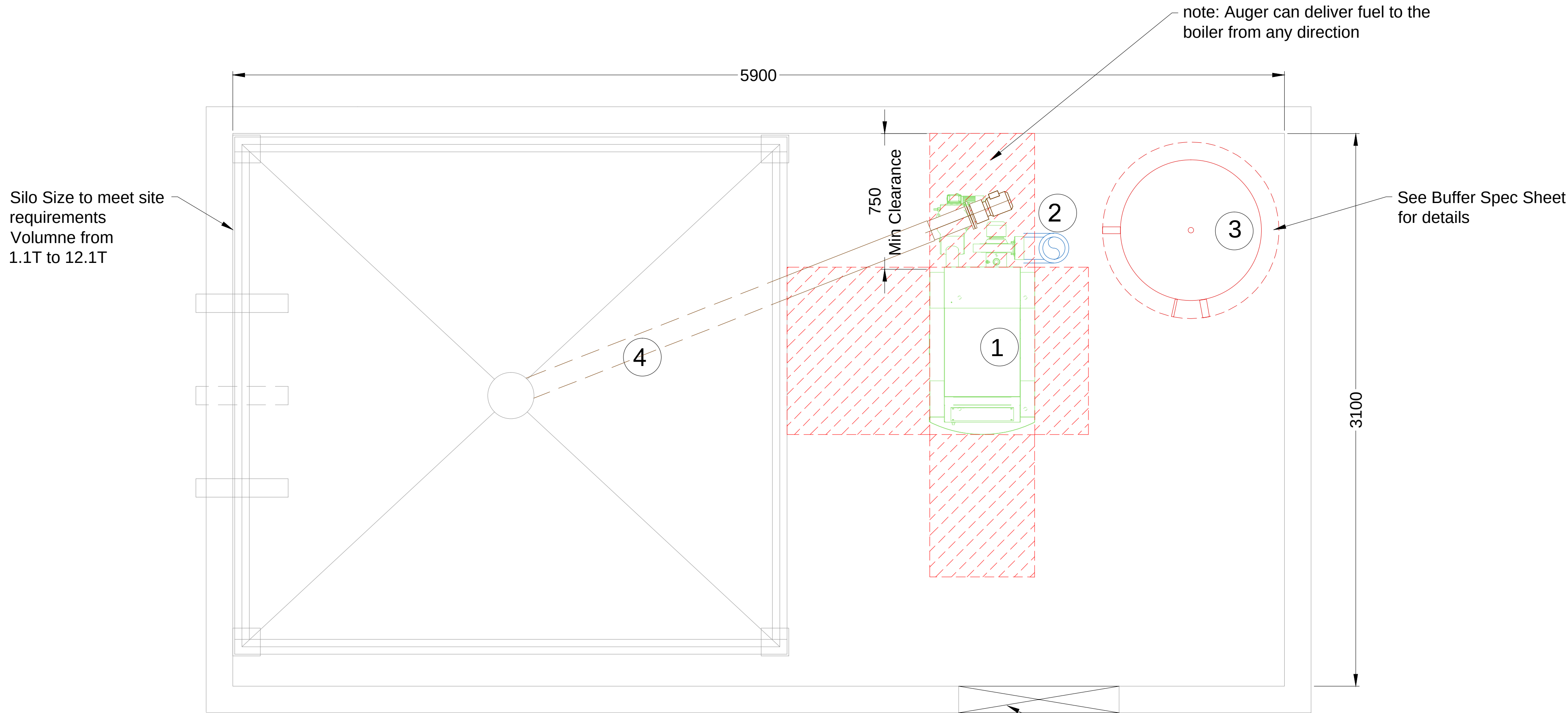
Plan View
